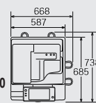
Sestava SR3150 + BU3070 PB3160
