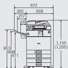
Sestava SH3070 PB3160
