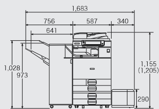
Sestava SR3160+ BU3070 PB3160 + RT3030
