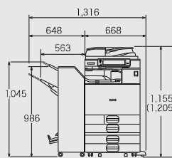
Sestava SR3150 + BU3070 PB3160
